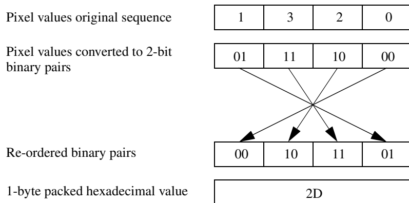
Figure 2-3 Packed Pixel Translation Example
